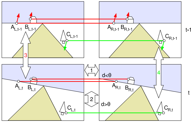
Fig. 2: Our approach consists of four steps that are performed for each new frame: (1) Sparse stereo and putative matching. (2) Separate the sparse flow by disparity based on the threshold \theta that adapts to the vehicle speed. (3) Recover the rotational component of the camera motion from two distant points A_t and B_t using RANSAC to robustly deal with outliers. (4) Recover the translational component of the camera motion from one close point C_t again using RANSAC.
