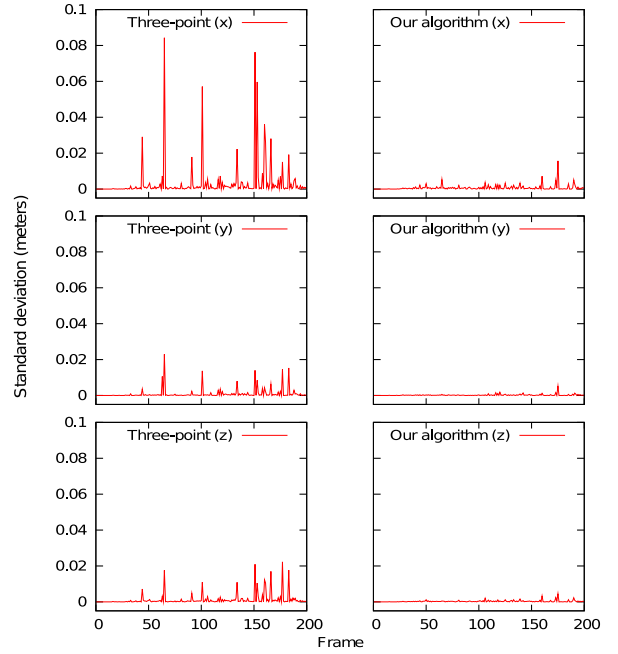
Fig. 4: Standard deviations for the x , y and z components of 15 runs over the first 200 frames of the San Antonio sequence for both the reference three-point algorithm (left column) and our algorithm (right column). While the three-point algorithm shows significant variation on some frames, our algorithm yields almost stable results, in agreement with Fig. 3.
